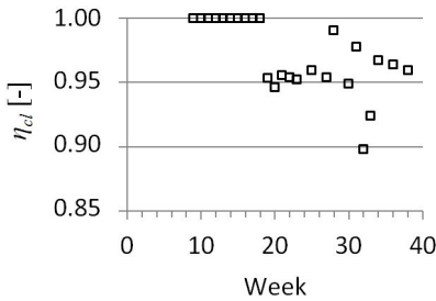
Fig. 10. Trash rack cleaning efficiency
