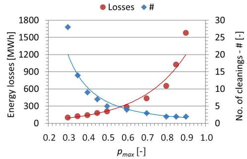
Fig. 11. Trash rack losses and number of cleanings necessary to keep the blockage factor below p_{max}
